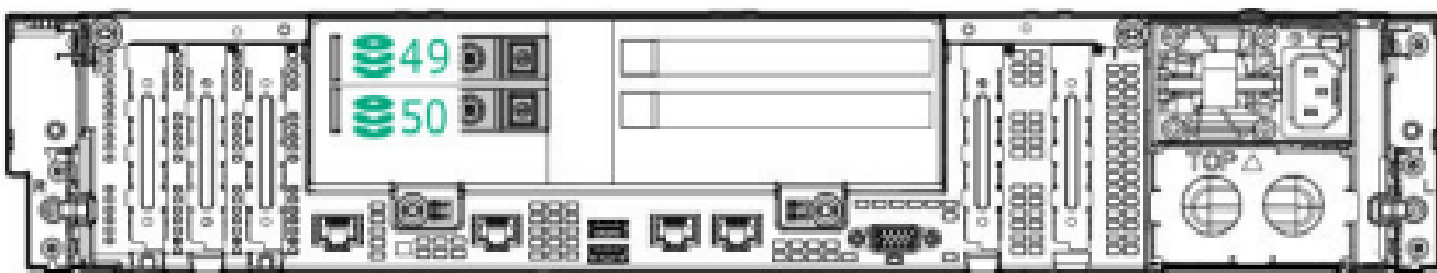
2SFF hot-plug rear drive numbering
